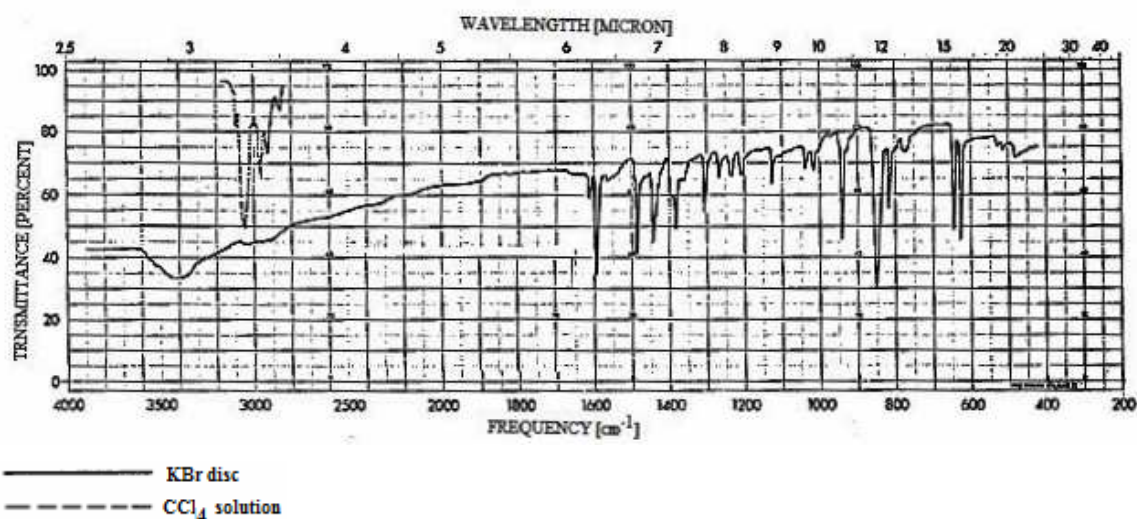
Figure-4: Infrared Spectrum of 1,7-naphthyridine (I)
