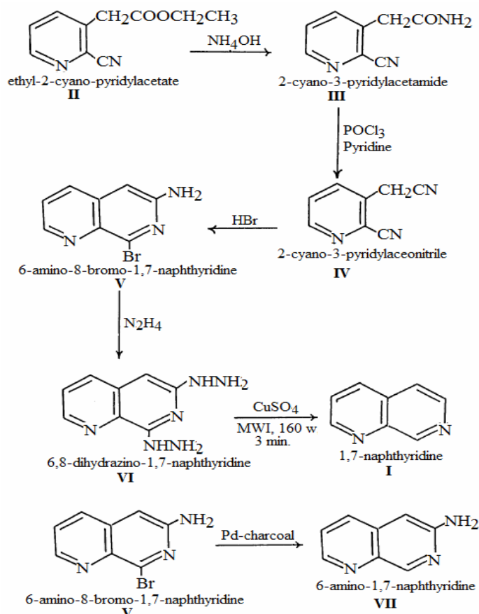
Scheme-1: Microwave assisted synthesis of 1,7-naphthyridines
