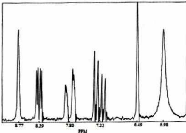
Figure-3: NMR Spectrum of 6-Amino-1,7-naphthyridine (VII) in DMSO-d 6
