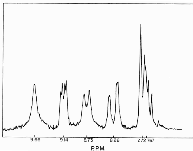
Figure-1: NMR Spectrum of 1,7-Naphthyridine (I) in \text{CDCl}_3
