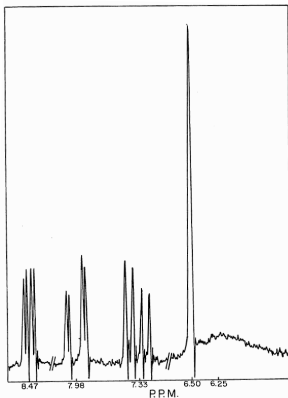
Figure-2: NMR Spectrum of 6-Amino-8-bromo-1,7-naphthyridine (VI) in \text{DMSO-d}_6
