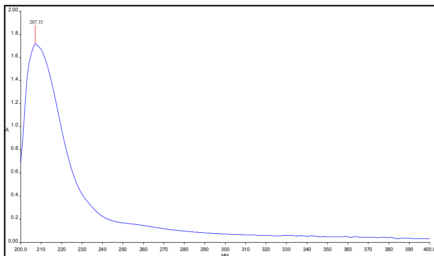
Fig.3. UV-VIS spectrum of silver nano particles using methanol as solvent.
