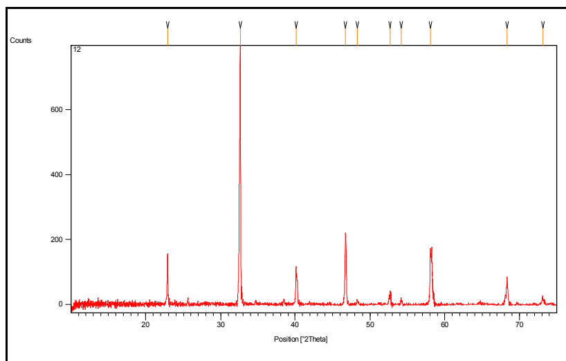
Fig.1. XRD spectrum for the silver nano particles.
