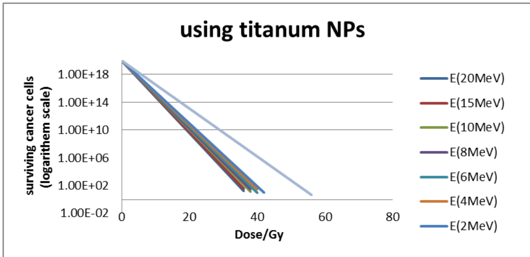
Figure 4: shows number of surviving cancer cells with and without titanium nano particles irradiate by x ray (2-20)MeV.
