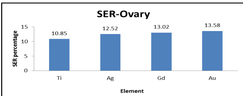
Figure 5: showimprovement in sensitivity enhancement ratio (SER) for ovary with using gold NPs, gadolinium NPs, silver NPs ad titanium NPs.
