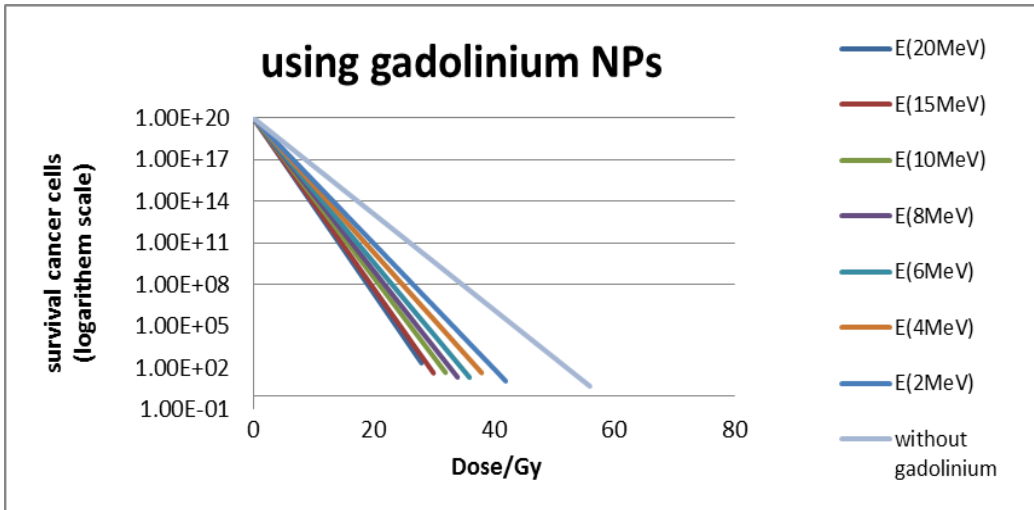
Figure 2: shows number of surviving cancer cells with and without gadolinium nano particles irradiate by x ray (2-20)MeV.
