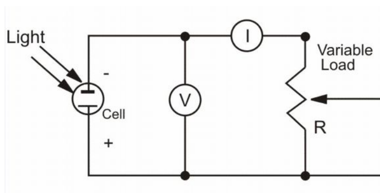
Fig.2 Experimental setup for measuring the current– voltage characteristics.
