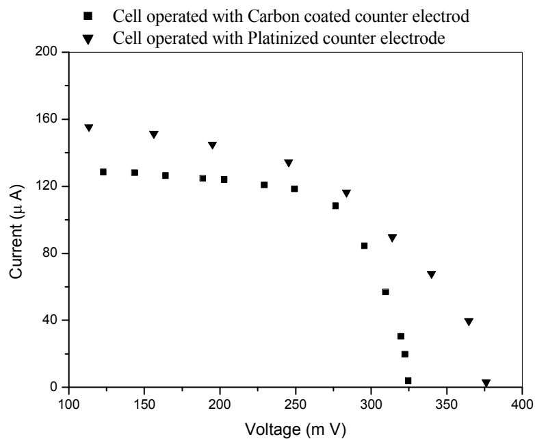
Fig.5 Photovoltaic response of fabricated DSSCs under illumination.
