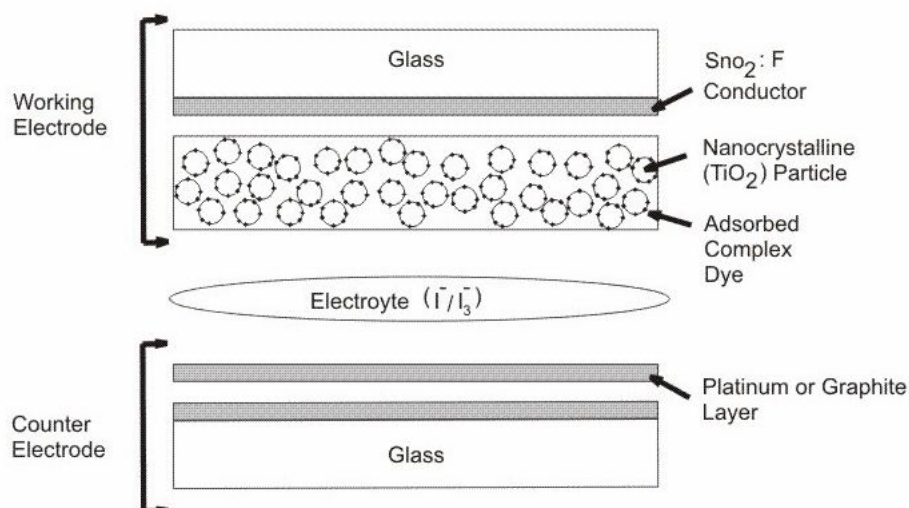
Fig.1 Schematic of a dye solar cell.
